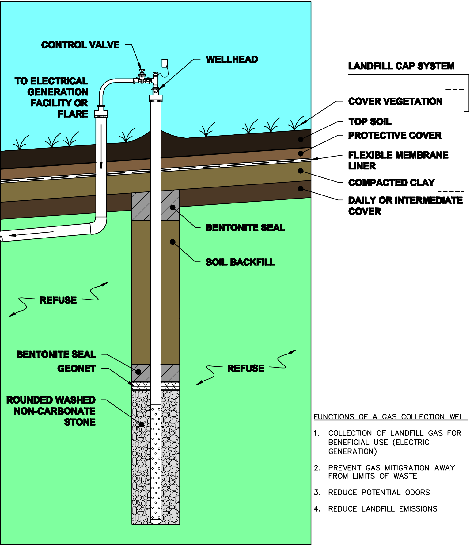
TYPICAL LANDFILL GAS COLLECTION WELL
